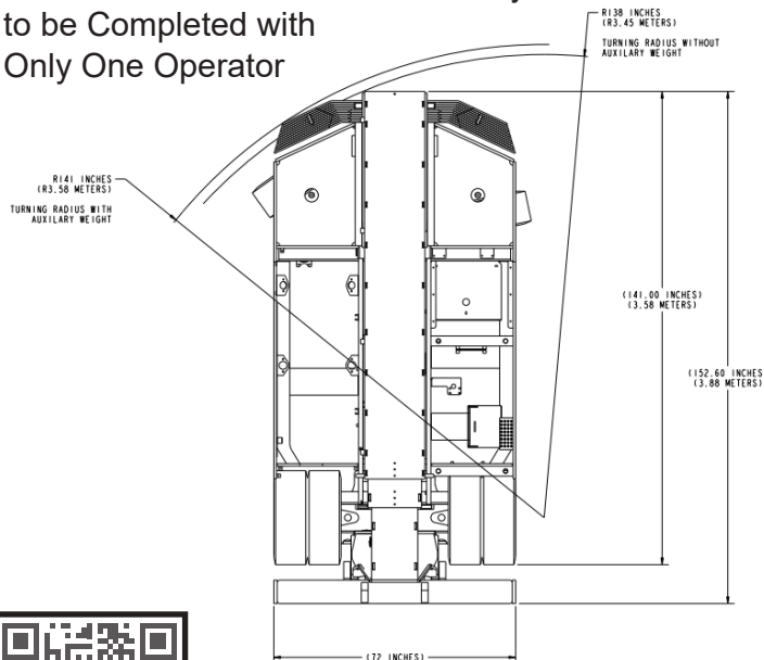
40,000 lb. (18,143.7kg) Capacity to 24" (609.6mm) Load Center
